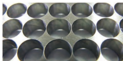
SUS304 湿式穿孔 S=1280 F=51 V=24.1 f=0.039
